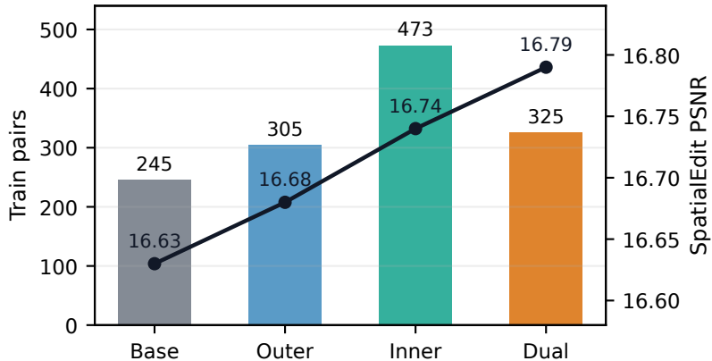
(a) Data evolution
