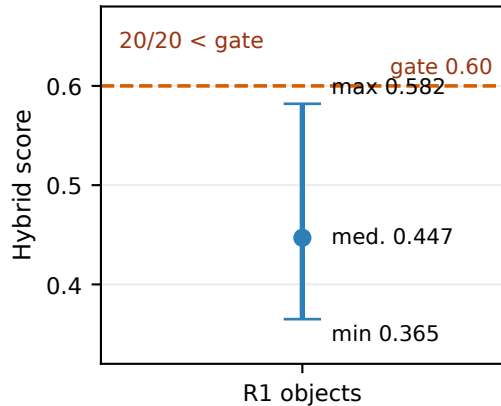
(b) Gate diagnosis
